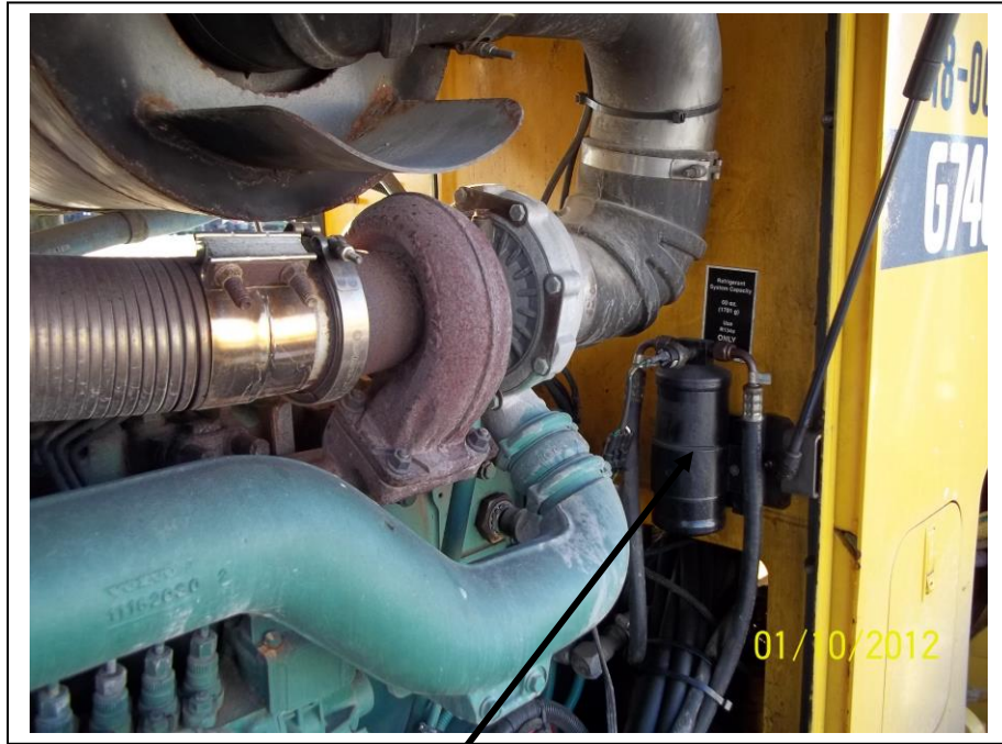
Mount the drier in this location
